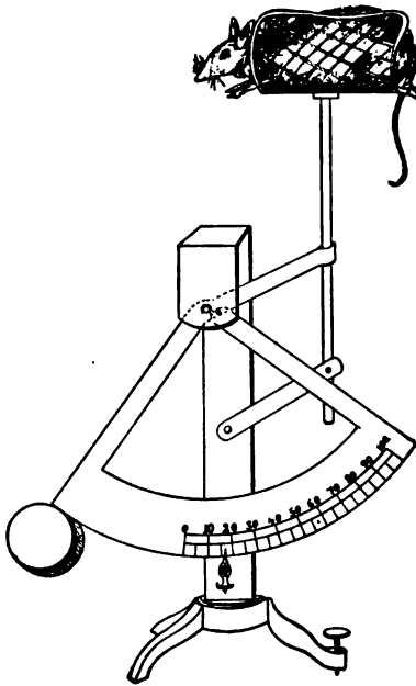
FIG. 167.—Mouse scales
